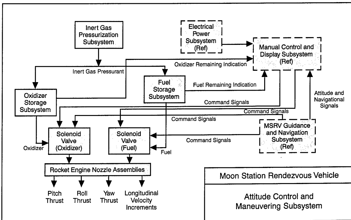
Figure 6-4. Schematic Block Diagram Example
