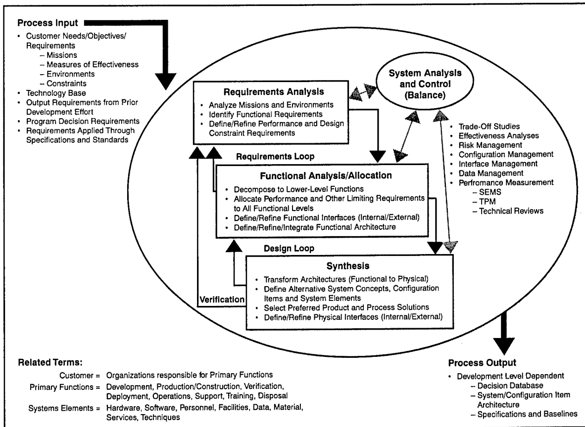
Figure 3-1. The Systems Engineering Process
