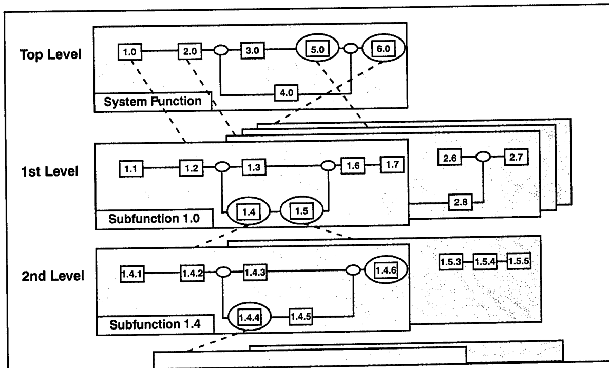
Figure 5-3. FFBD Traceability and Indenture
