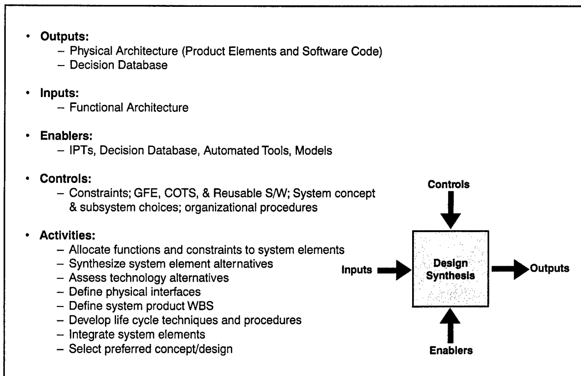
Figure 6-1. Design Synthesis
