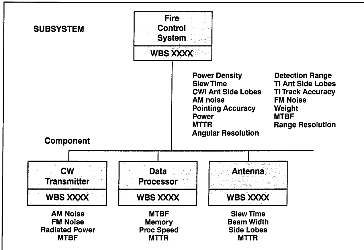
Figure 14-3. Shipboard Fire Control System (Partial)
