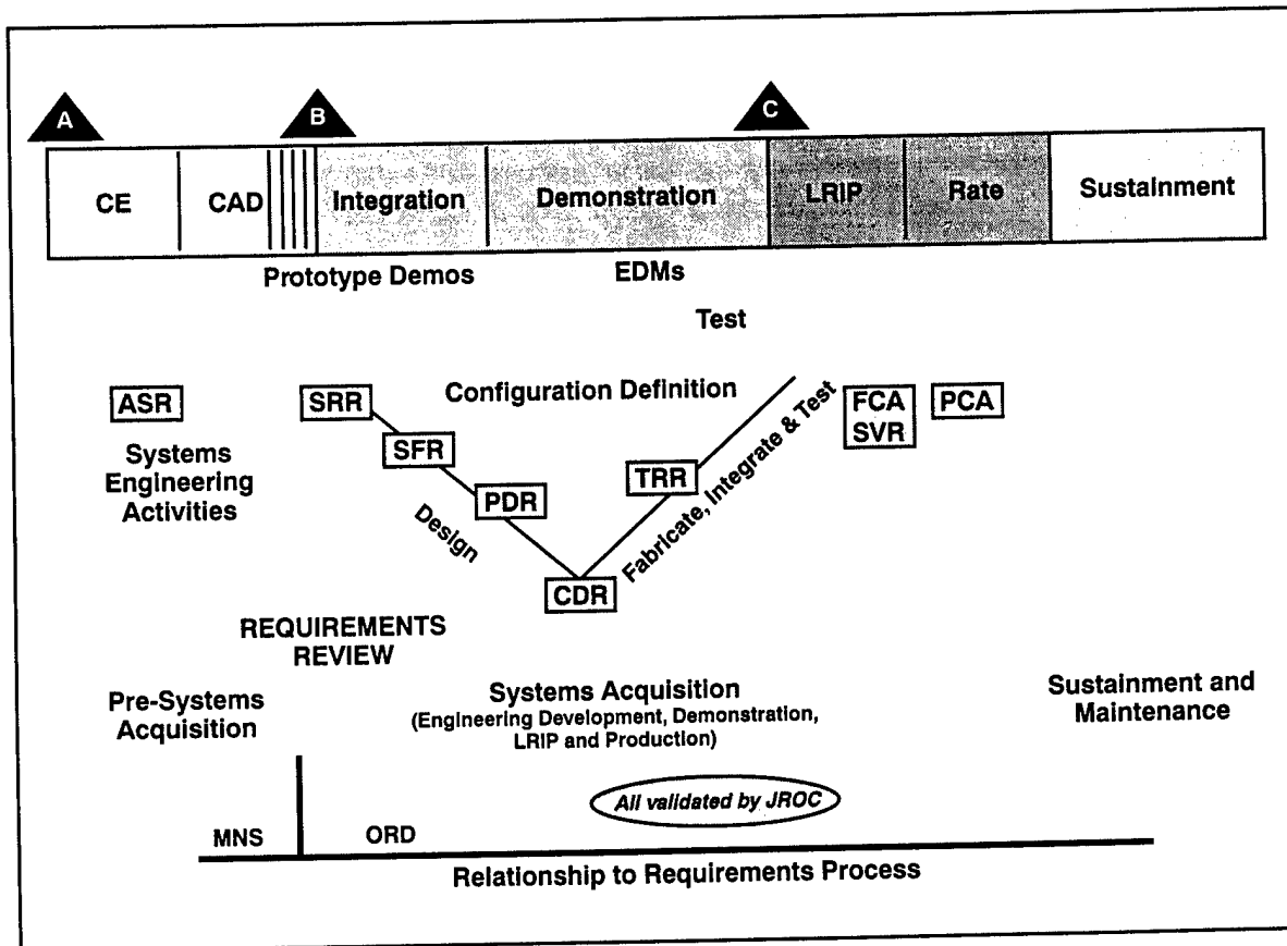
Figure 11-4. Relationship of Systems Engineering Events to Acquisition Life Cycle Phases
