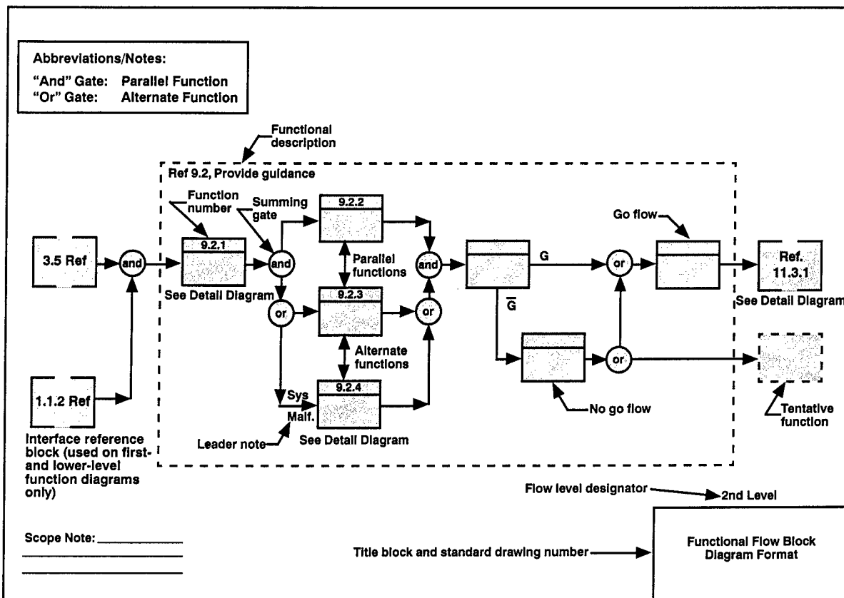
Figure 5-4. Functional Flow Block Diagrams (FFBD) Format
