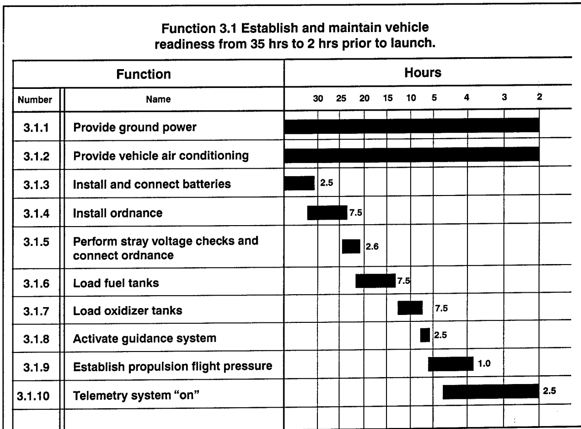
Figure 5-8. Time Analysis Sheet
