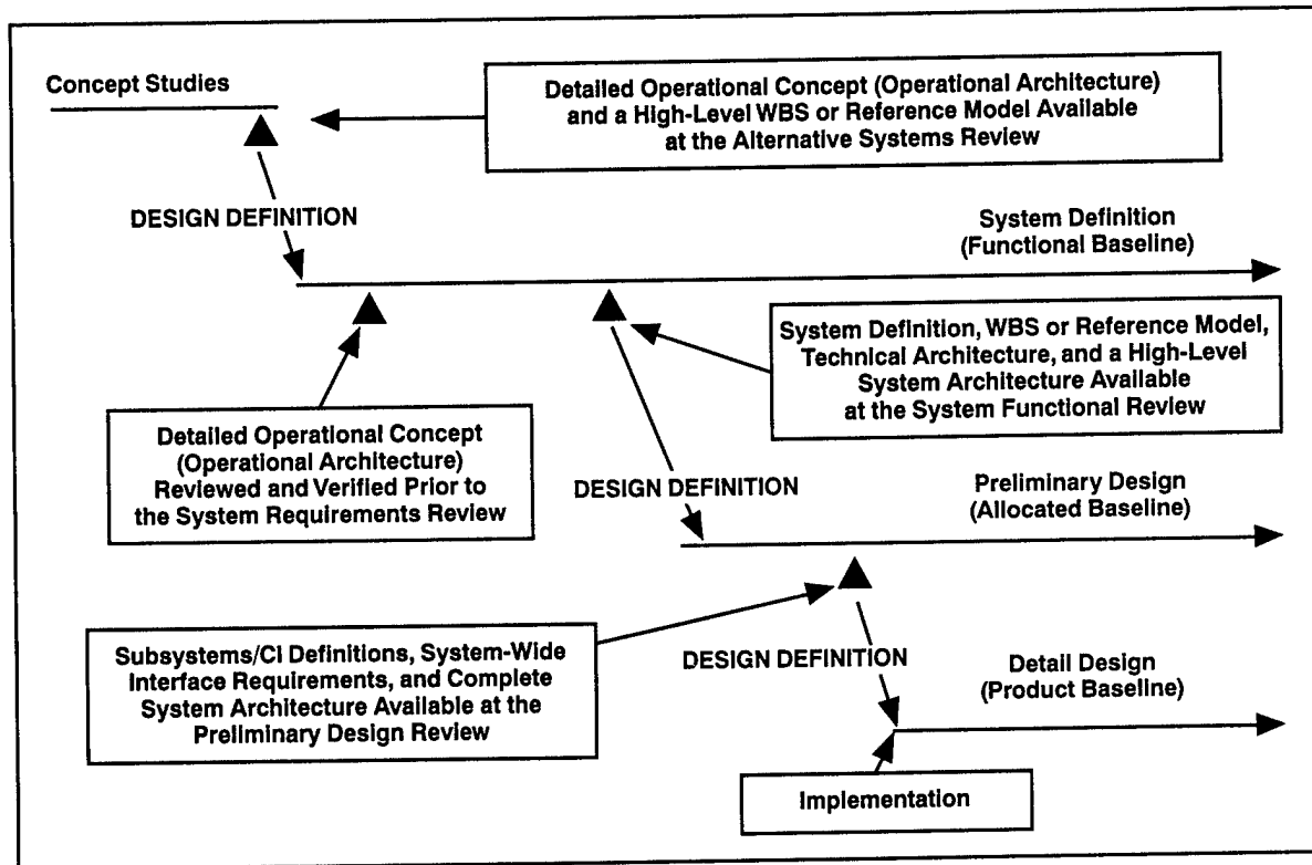
Figure 17-7. Phasing of Open System Development
