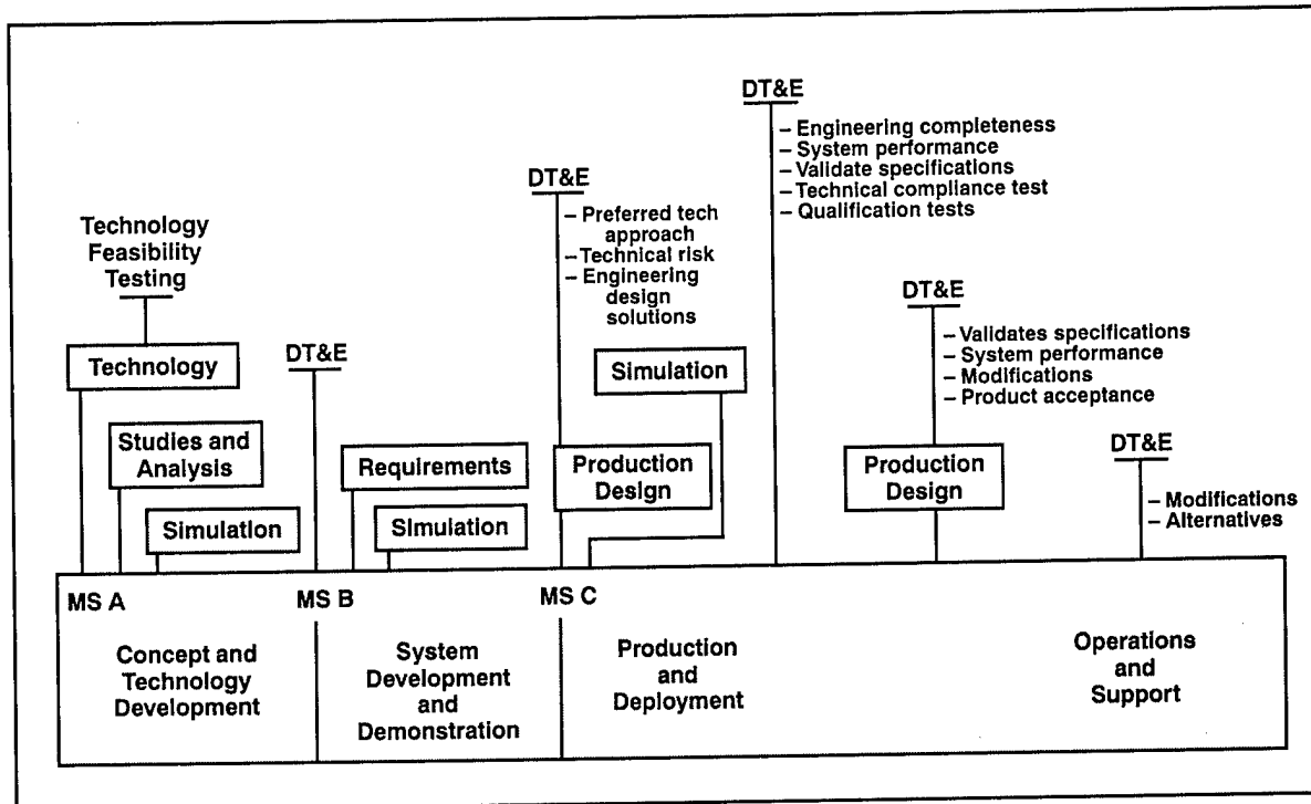
Figure 7-3. DT&E During System Acquisition
