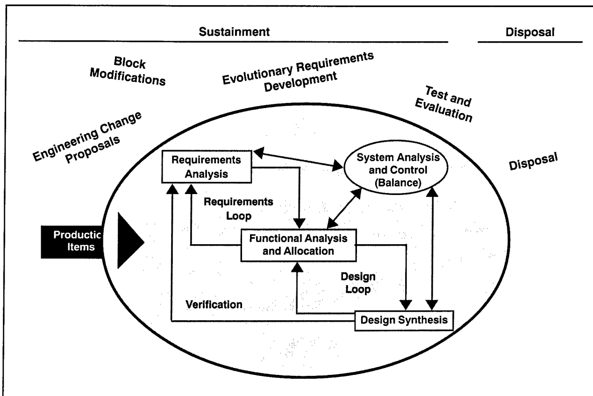
Figure 2-7. Sustainment and Disposal
