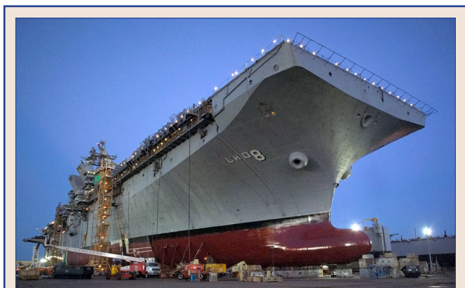
A bow view of the USS Makin Island (LHD 8) under construction in Pascagoula, Miss. The USS Makin Island is the Navy's first amphibious assault ship equipped with an all electric auxiliary system and a hybrid gas turbine - electric propulsion system. On her maiden voyage, her hybrid drive saved approximately one million gallons of fuel and is expected to save more than $250 million over her lifecycle. (Photo by Mr. Steve Blount, Pascagoula, Miss.)
