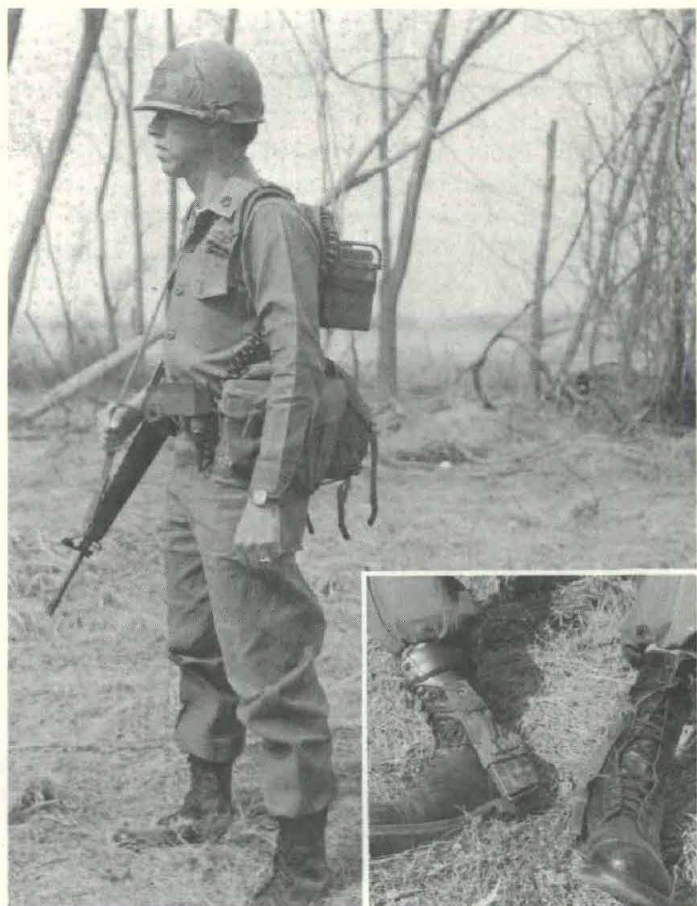
COMBAT SOLDIER displays AN/PSN-7 Land Navigator System. Inset shows coils attached to the boots of the operator.
