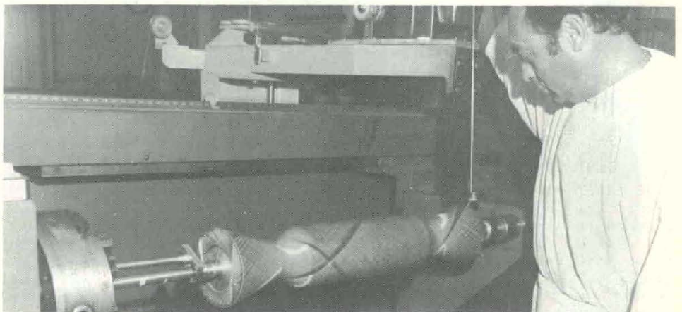
Fig. 3. WINDING of WECOM recoilless nozzles. Each complete winding operation produces two nozzles for the U.S. Army's new Advanced Light Antitank Weapon.
