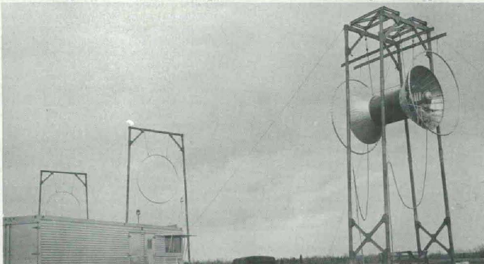
TEMPS 7,000,000-volt pulse generator (right background) is elevated 65 feet above ground and connected to an antenna arrangement (left background). The generator can radiate electromagnetic waves over 150 feet. The control panels are installed inside the van.
