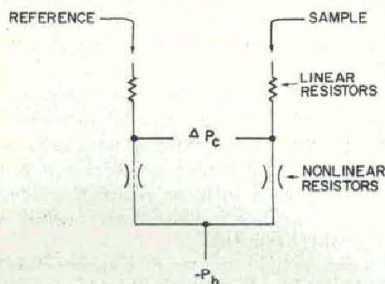
Fig. 1. Fluidic resistor bridge concentration sensor
