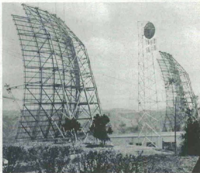
TROPOSPHERIC-SCATTER communications system on Mt. Luay speeds messages over 300 miles in Hawaiian network.
