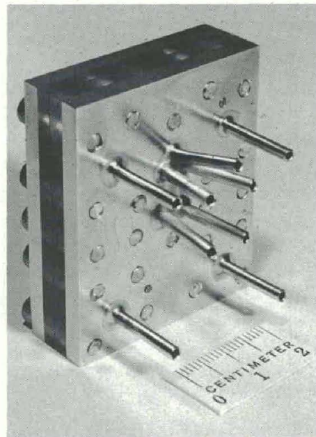
Fig. 2. Experimental hardware
