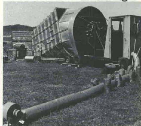
WIND TUNNEL, simulating firing conditions during aircraft flight, was used to study infrared radiation from hot weapons.
